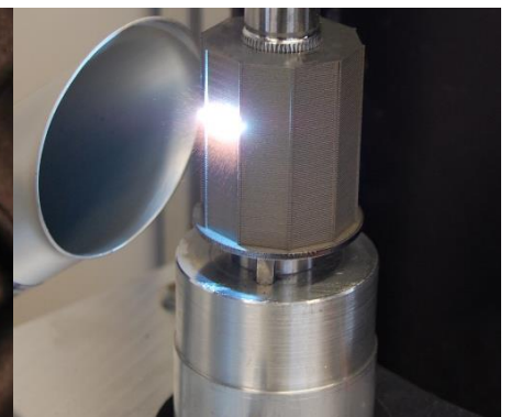
Laser processing of a rotor
